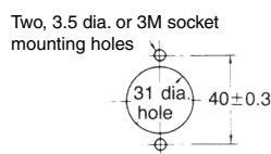
Mounting Holes
